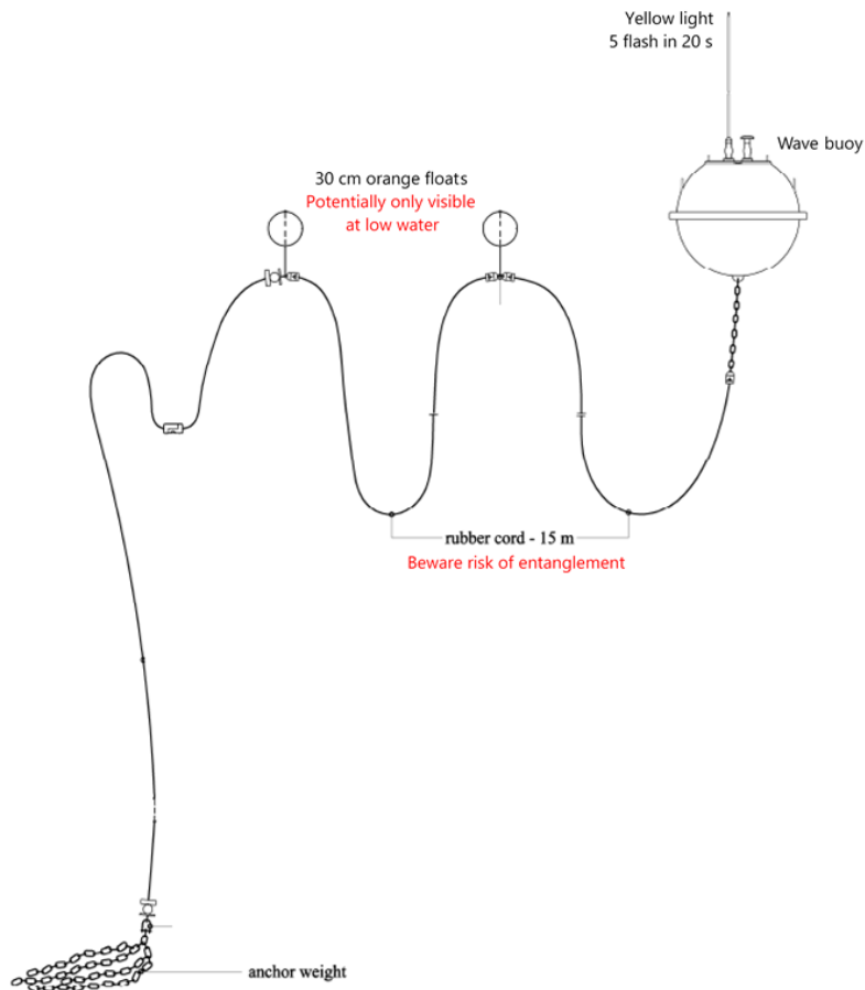
Figure 1: Lowestoft Wave Buoy
