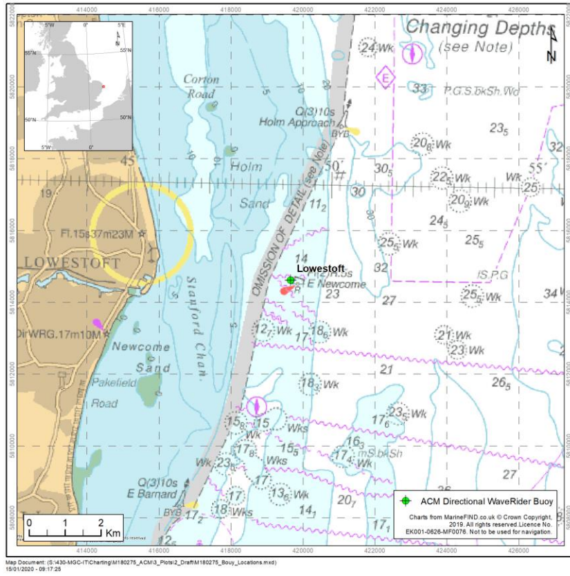
Figure 1: Lowestoft Wave Buoy
