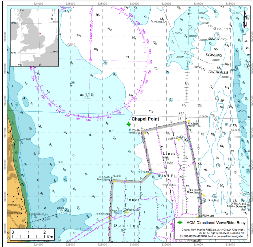
Figure 1: Chapel Point Wave Buoy
