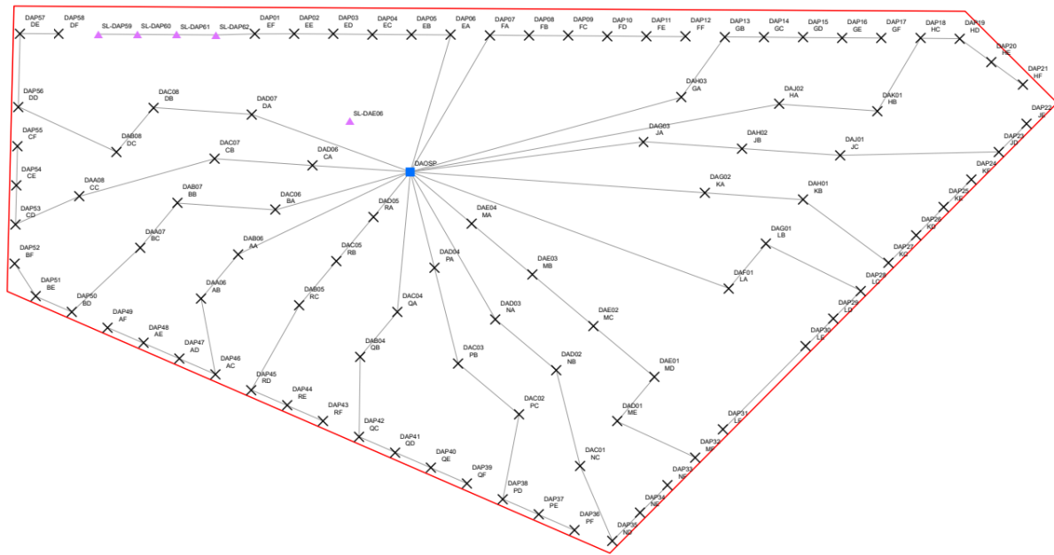
Figure 1: Dogger Bank A OWF Array Area and WTG Layout
