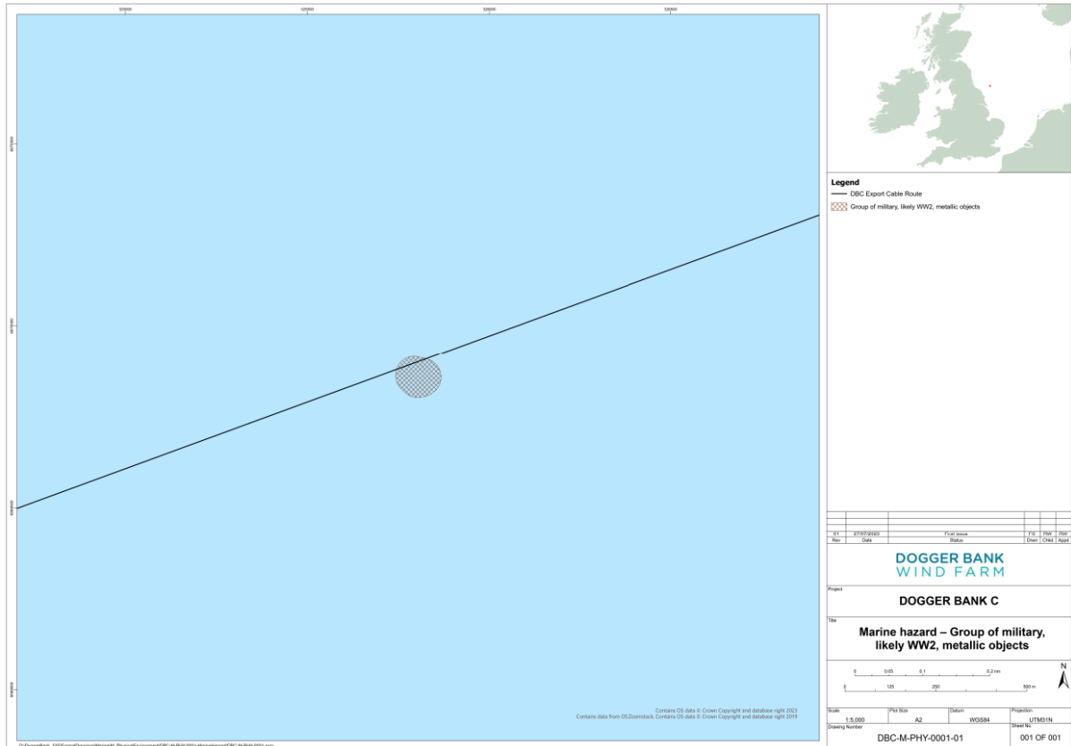
Figure 1: Position of Marine Hazard in the Dogger Bank C Export Cable Corridor
