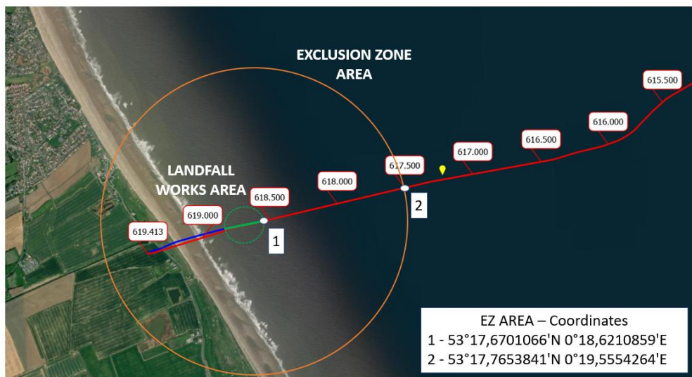
Figure 1 – Guard Vessel location, work area and EZ
