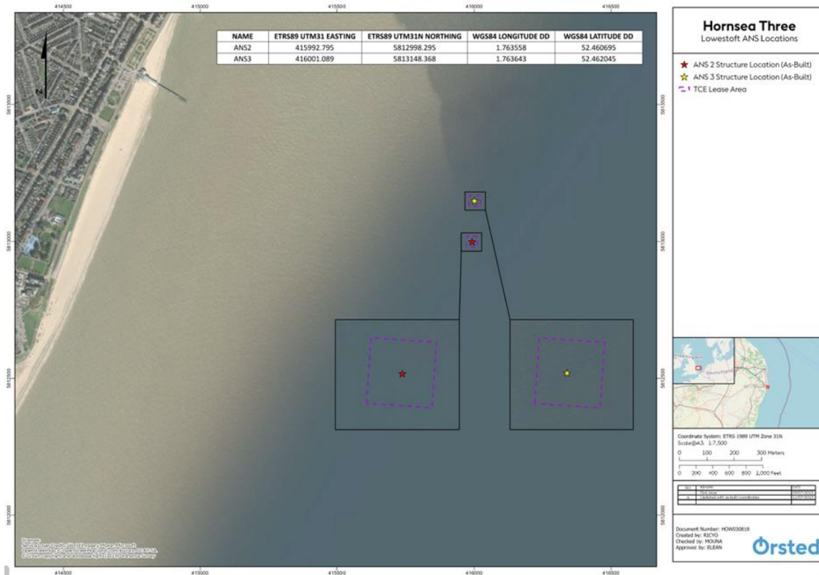
Figure 1: Hornsea Three Work Area – Lowestoft ANS2 and ANS3
