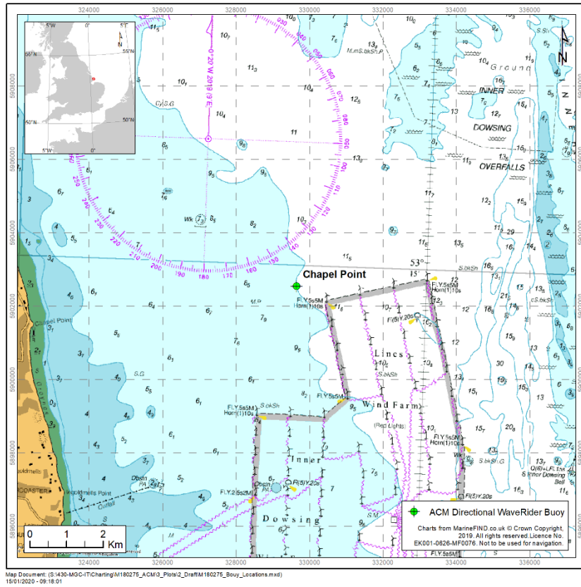
Figure 1: Chapel Point Wave Buoy
