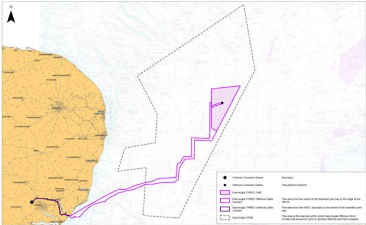
Figure 1: East Anglia 3 Cable Installation Working Area Overview.
