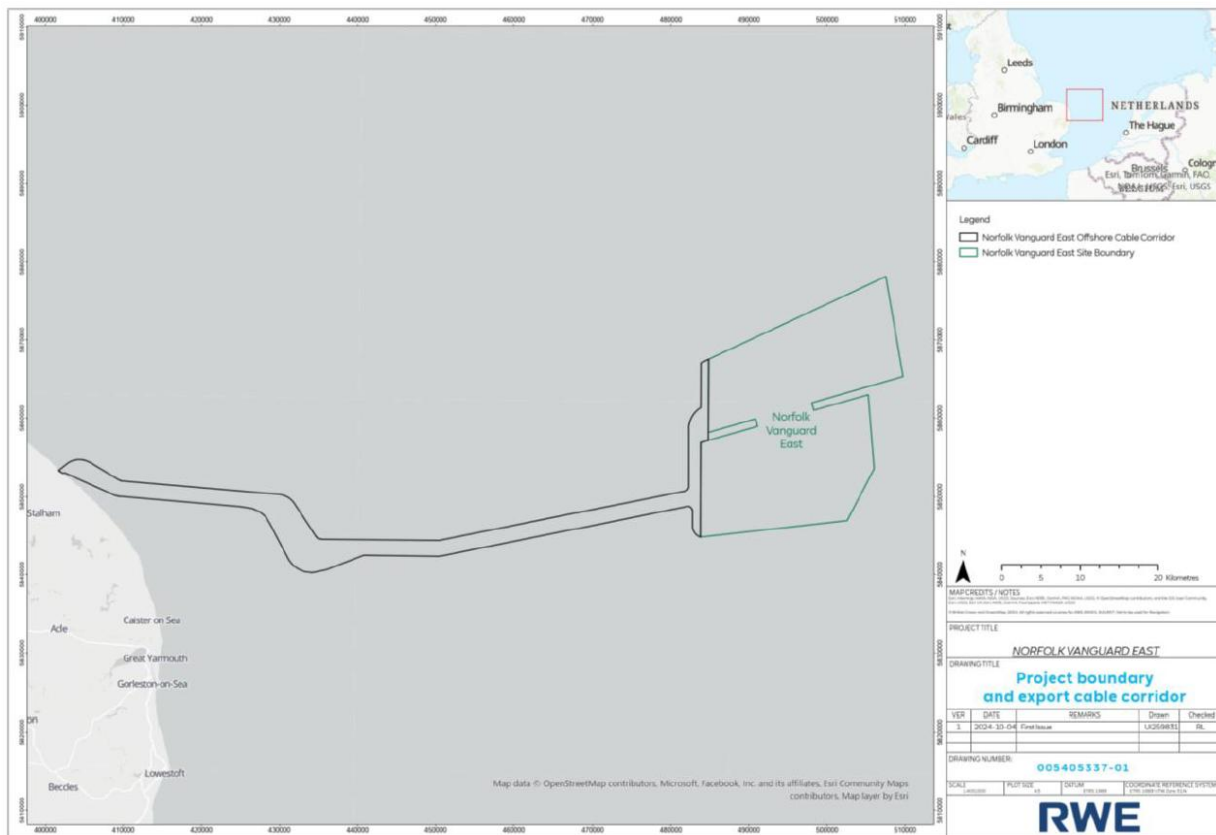
Figure 1. General working area.
