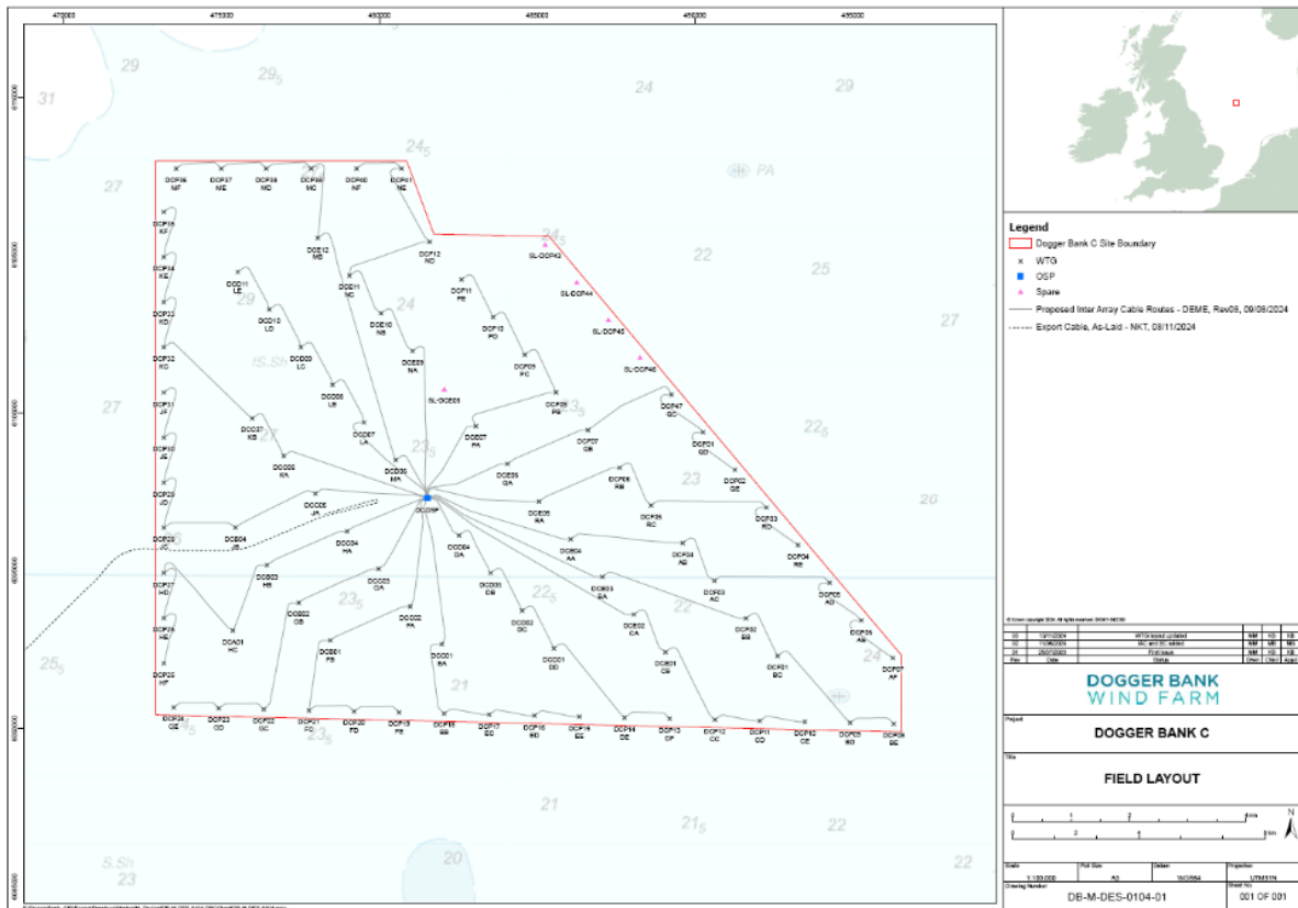
Figure 1: Dogger Bank C OWF WTG Foundation locations and IA Cable Layout
